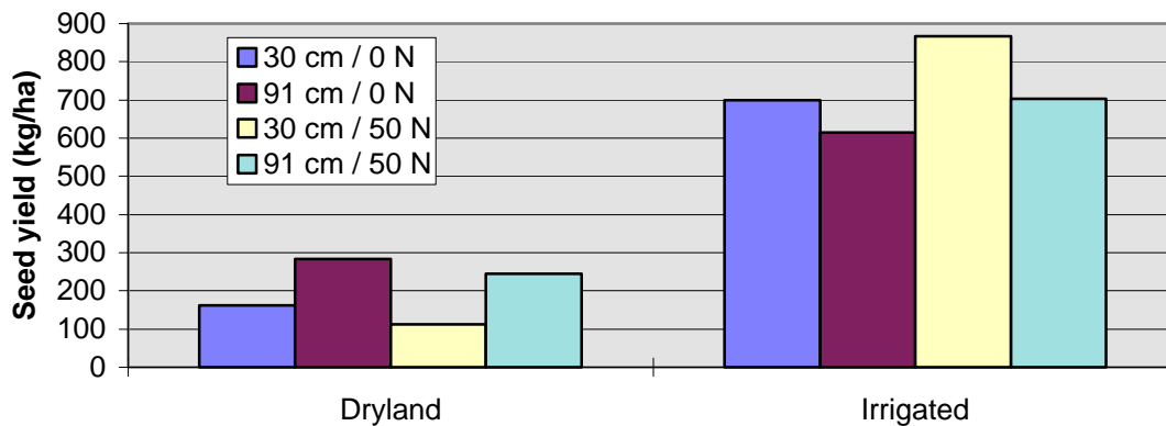
Figure 2: Effect of row spacing, N fertility and irrigation on seed yield of slender wheatgrass at Scott (Crowle, 1966)
